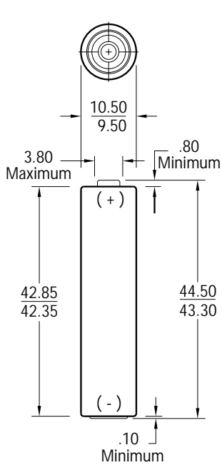
Dimensions (mm)
