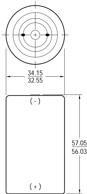
Dimensions (mm)
