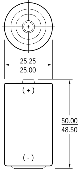
Dimensions (mm)
